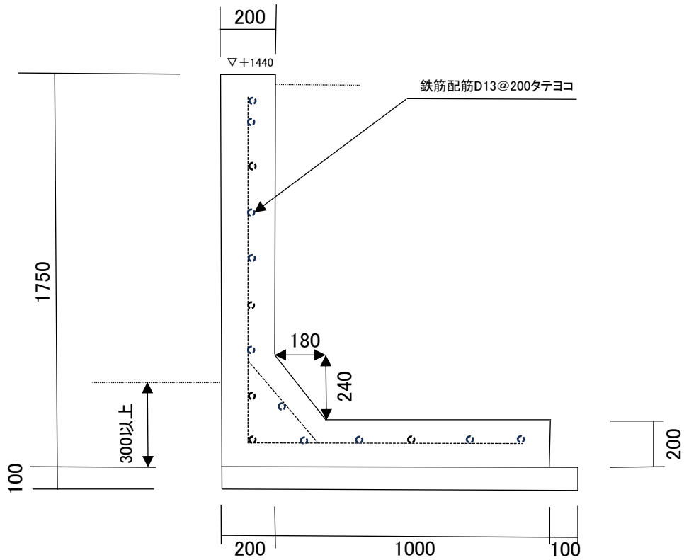
② L型擁壁工 L=6.7m
